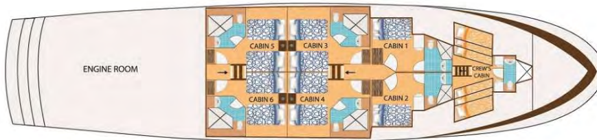
LOWER DECK
